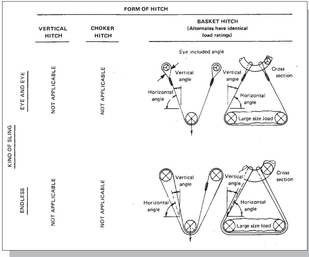
Figure 4.1-3 Rope Sling Configurations with Angled Legs
