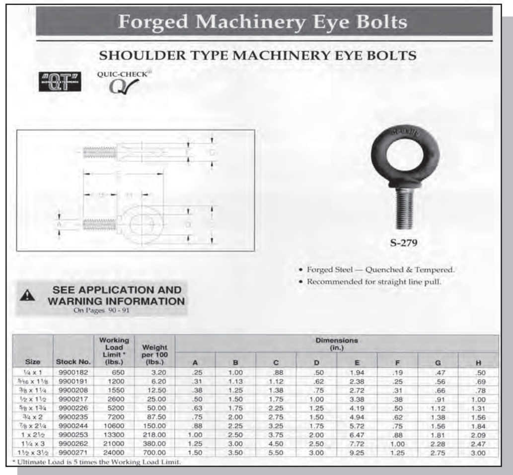
Figure 4.2-25 Eye Bolts
