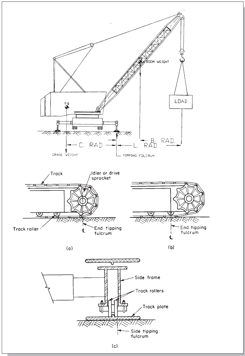
Figure 3.7-1 Tipping Fulcrum for Truck and Hydraulic Cranes
