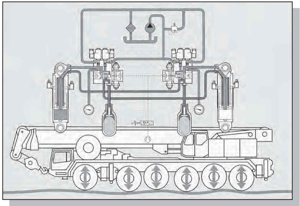
Figure 3.5-3 All Terrain Suspension, Top Shows Schematic of Hydraulic Suspension for One "Axle"
