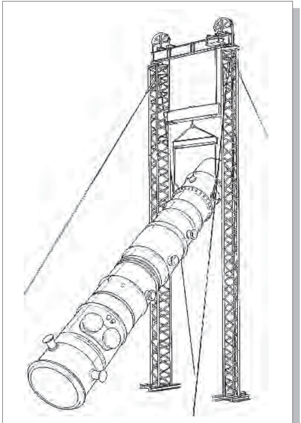
Figure 5.7-1 Gallows Pole Arrangement
